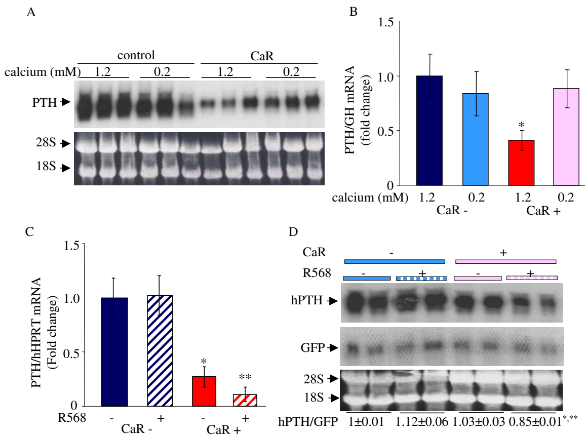
Figure 5 Expression of the CaR decreases PTH mRNA levels and confers responsiveness to a low [Ca^{2+}]_o and the calcimimetic R568. A. Representative Northern blot analysis for PTH mRNA in cells transiently transfected in triplicate with hPTH and either the CaR plasmid or empty vector. After transfection cells were grown in 1.2 or 0.2 mM Ca^{2+} medium for an additional 48 h. Ethidium bromide staining of the membrane is shown as loading control. B. qRT PCR for PTH corrected for co-transfected GH mRNAs for cells treated as in A. C. qPCR for PTH and HPRT mRNAs from cells expressing the hPTH gene and the CaR (CaR+) or empty vector (CaR-) in cells grown in 1.2 mM Ca^{2+} supplemented with either R568 or vehicle. The results in A-C represent one of three repeat experiments performed in triplicate with similar results. D. Representative Northern blot for PTH and GFP mRNA levels in cells transfected with PTH and GFP and either CaR (CaR+) or empty vector (CaR-). The cells were grown in 0.2 mM calcium supplemented with R568 or vehicle. Quantification of the results is shown below the gel. The results are presented as mean \pm SE of two repeat experiments performed in triplicate. *, P < 0.05 , CaR+:CaR-; **, P < 0.05 , CaR+, treated:CaR+, untreated.
