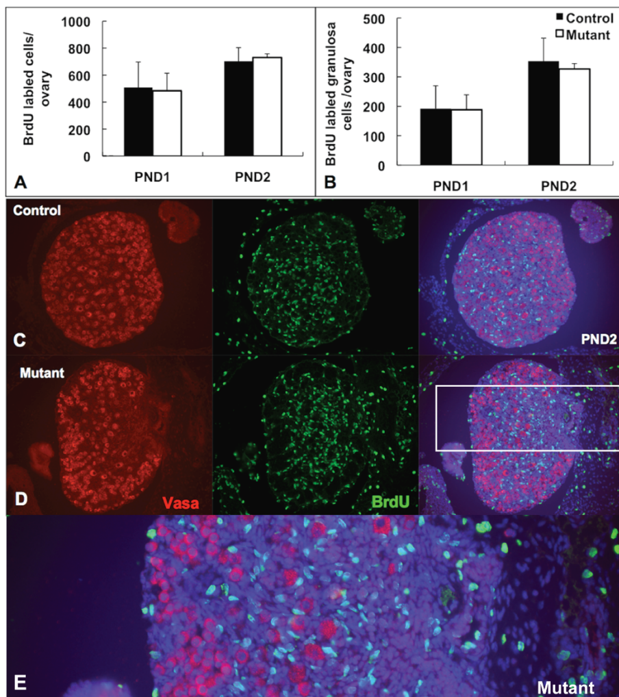
Figure 6 Absence of extended cell proliferation in neonatal Amhr2-Cre/+;Notch2 flox/- ovaries. (A, B) Quantification of (A) total 5-bromo-2'-deoxyuridine (BrdU)-positive cells and (B) BrdU-positive pre-granulosa/granulosa cells (defined as a BrdU-positive somatic cell adjacent to a Vasa-positive oocyte). Ovaries were harvested from Amhr2-Cre/+;Notch2 flox/- and control littermate mice after a 2-hour BrdU pulse administration on postnatal day (PND)1 or PND2. Data are presented as the mean \pm SD of four ovaries from four individual mutant or control mice. There were no significant differences in the numbers of either (A) total proliferating cells or (B) proliferating pre-granulosa/granulosa cells between the control and the Amhr2-Cre/+;Notch2 flox/- ovaries. (C, D) Representative micrographs showing BrdU incorporation from (C) control littermate and (D) Amhr2-Cre/+;Notch2 flox/- ovaries at PND1. No oocyte in either (C) the control or (D) mutant ovary incorporated BrdU. BrdU-positive cells are in green; oocytes are in red (Vasa-positive), with nuclear DAPI staining in blue. (E) Higher magnification view of the mutant ovary (boxed region in D).
