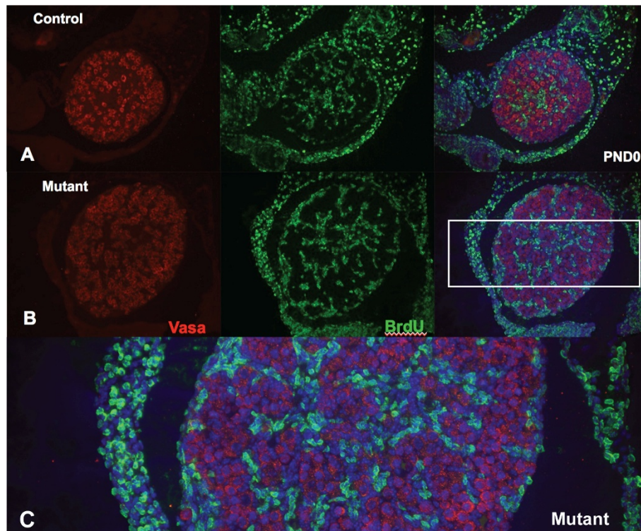
Figure 5 Absence of extended oocyte proliferation in embryonic Amhr2-Cre/+;Notch2 fllox/- ovaries. Pregnant mice were injected with 5-bromo-2'-deoxyuridine (BrdU) twice daily between E16.5 through E18.5 (a total of six injections). Ovaries were isolated from Amhr2-Cre/+;Notch2 fllox/- and control littermate progeny on the day of birth (postnatal day 0; PND0), and sections were stained with anti-Vasa (red) antibodies to label oocytes, and with anti-BrdU (green) antibodies to identify proliferating cells. Sections were also counterstained with DAPI (blue) to stain cell nuclei. As shown in the merged figure on the right, at PND0, no oocyte in either (A) littermate control or (B) mutant ovaries had incorporated BrdU as a result of these injections. (C) Higher magnification view of the mutant ovary (boxed region in B).
