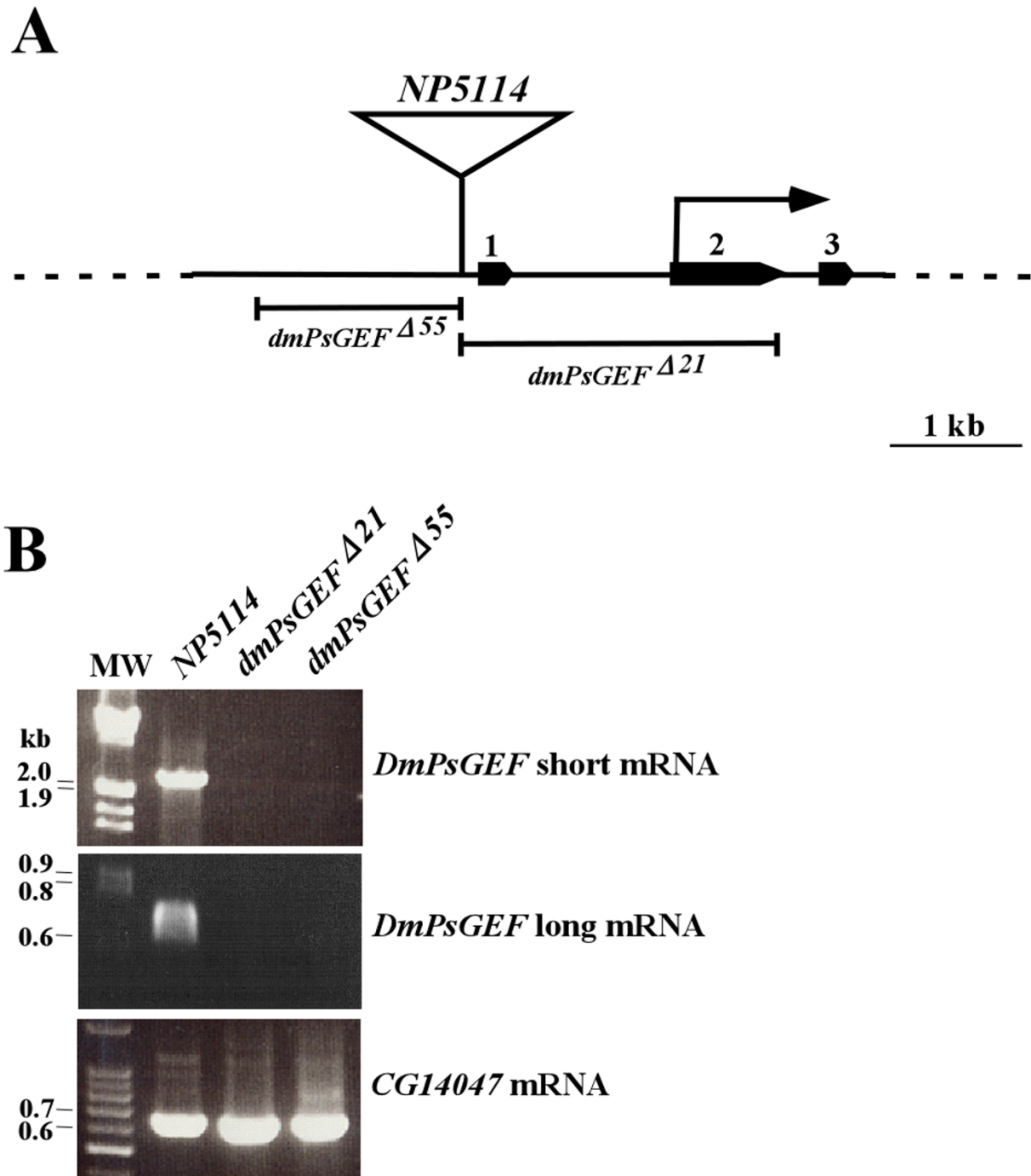
Figure 5 Generation of DmPsGEF deletion mutants and DmPsGEF mRNA expression analysis in the mutants. (A) NP5114 is located at 5' upstream of exon 1 of DmPsGEF , and translation is initiated at exon 2 (arrow). Exons 1 to 3 are indicated by solid pentagons. Two DmPsGEF deletion mutants ( dmPsGEF \Delta 55 and dmPsGEF \Delta 21 ) were generated by imprecise excision of NP5114 , and the deleted genomic region in each mutant is also shown. The scale bar indicates 1 kb. (B) The expression of short and long DmPsGEF mRNAs as well as CG14047 mRNA in NP5114 , dmPsGEF \Delta 21 , and dmPsGEF \Delta 55 embryos was examined by reverse transcriptase-polymerase chain reaction. Both short and long DmPsGEF mRNAs are present in the parent NP5114 but not in dmPsGEF \Delta 21 and dmPsGEF \Delta 55 embryos, while CG14047 mRNA is present in all genotypes of embryos. The numbers at left side of the panels indicate the sizes of bands (in kb) in molecular weight markers (MW).
