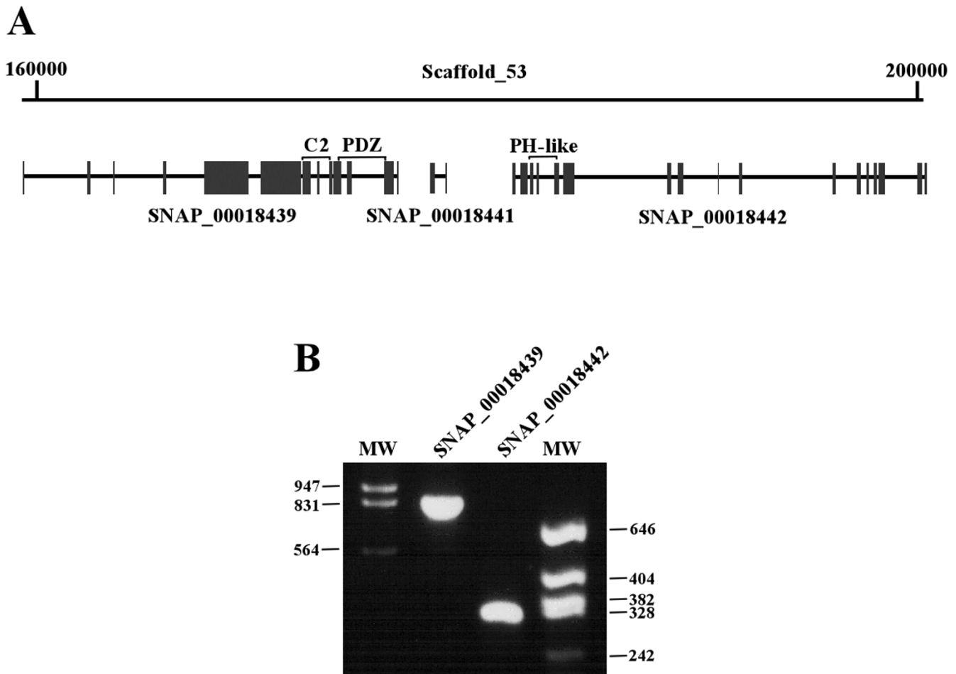
Figure 3 Daphnia pulex genomic DNA region containing PsGEF and mRNA expression of Daphnia PsGEF and neighboring genes. (A) Daphnia PsGEF is located in scaffold 53 of the genome assembly. The predicted transcript SNAP_00018439 encodes PsGEF containing the C2 and PDZ domains. The neighboring transcripts SNAP_00018441 and SNAP_00018442 encode a novel short protein and a protein with a PH-like domain, respectively. The predicted exons are indicated by the solid rectangles. The exons encoding the C2, PDZ, and PH-like domains are indicated by brackets. The exons encoding the RhoGEF domain are not present in this scaffold. (B) The expression of SNAP_00018439 and SNAP_00018442 mRNAs in Daphnia is confirmed by using RT-PCR. However, SNAP_00018441 mRNA can not be detected by this analysis. The numbers at both sides of the panel indicate the sizes of bands in molecular weight markers (MW).
